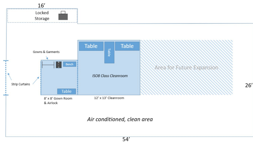
Figure 24 Rocket Lab's Long Beach Payload Processing Facility layout
